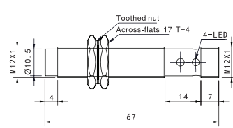
TRN12-04□□-E2
