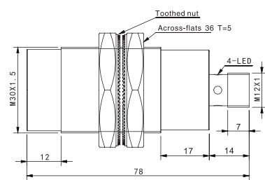
TRN30-15□□-E2
