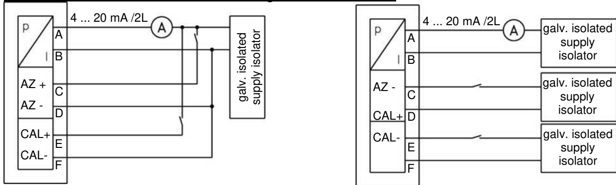
Fig. 3 Diagrams circuit
